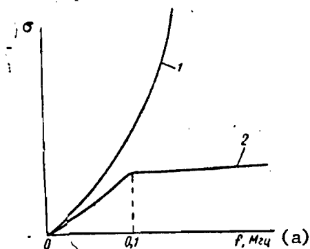
Figure 25. Dependence of the attenuation \sigma of the shielding on the frequency of electromagnetic oscillations. 1 -- for a shield of continuous material; 2 -- for a lattice shield.
