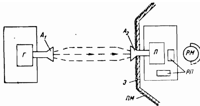
Figure 32. Scheme for tuning a radar antenna with application of an umbrella shield for protection from irradiation (top view). З -- shield; ПМ -- absorbing material; PM -- work area; Г -- generator; П -- receiver.
