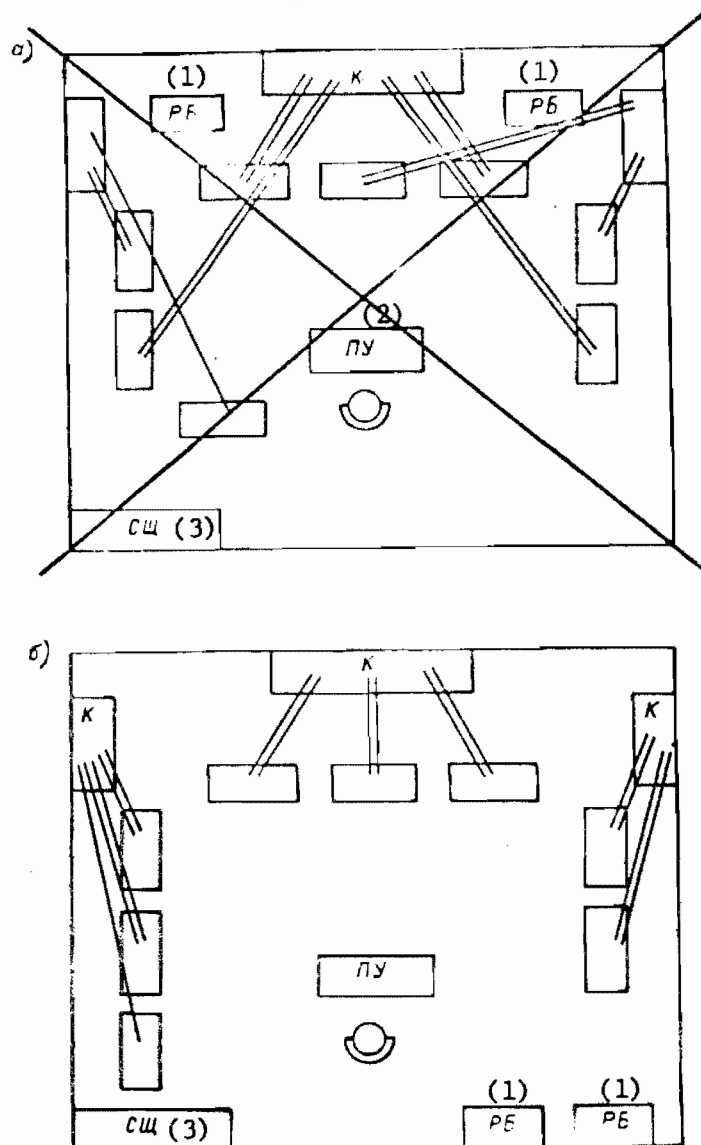
Figure 42. Placement of transmitters and feeder lines in the transmitting center of the shipping line. K -- commutators; ПБ -- power board
