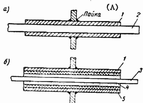
Figure 35. Leads of control arms through the walls of a shielding chamber: a -- lead of an arm made of dielectric; b -- lead of a metal arm. 1 -- metal tube; 2 -- dielectric axis; 3 -- metal axis; 4 -- absorbing material; 5 -- dielectric.
